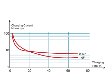
Figure 49. LV Series - 10 Volt Charge
