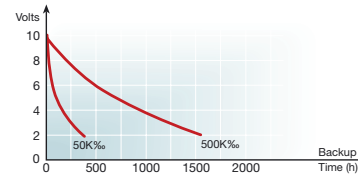
Figure 39. 5.0F - LV Series
