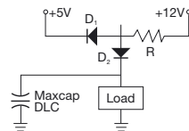
Figure 58. Voltage Clamping Arrangement
