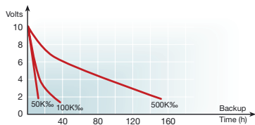
Figure 31. 0.47F - LV Series
