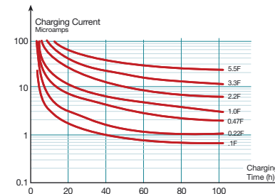
Figure 51. LJ Series - 5 Volt Charge
