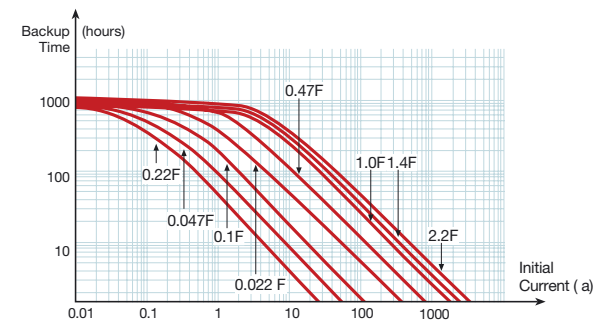
Figure 6. Minimum Backup Time Versus Initial Current for CMOS RAM Applications Using Maxcap DLC LC, LK, LX, LJ and LT Series from 5 to 2 Volts at 25°C
