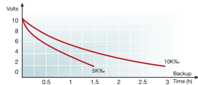
Figure 30. 0.47F - LV Series
