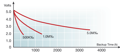
Figure 24. 3.3F - LJ Series
