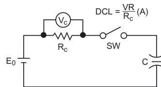
Figure 4. DC Leakage Current (Charging Current – 30 Minute)
