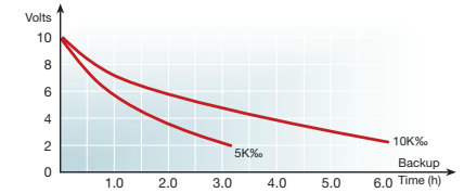
Figure 34. 1.0F - LV Series
