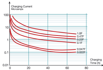
Figure 47. LK Series - 5 Volt Charge
