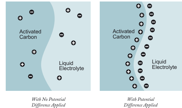
Figure 64. Electric Double Layer Principle
