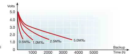
Figure 20. 1.4F – LC Series Only
