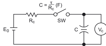
Figure 1. Capacitance – Charge Method
