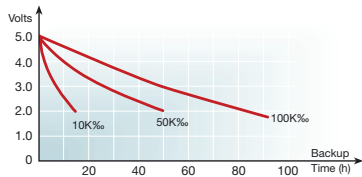
Figure 23. 3.3F - LJ Series
