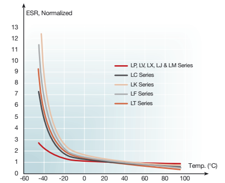
Figure 54. ESR Versus Temperature - 1.0F Capacitors
