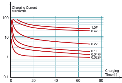
Figure 44. LP Series - 5 Volt Charge
