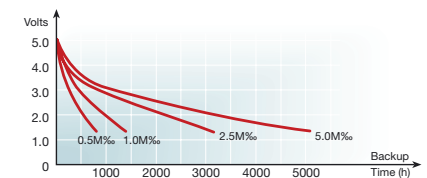
Figure 22. 2.2F – LC, LX, LJ Series
