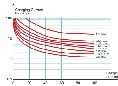
Figure 52. LM Series - 5 and 3.5 Volt Charge
