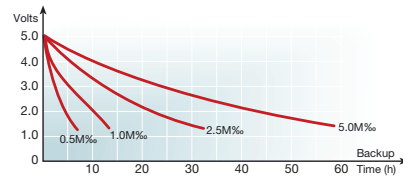
Figure 8. 0.022F – LC, LK, LT, LX Series
