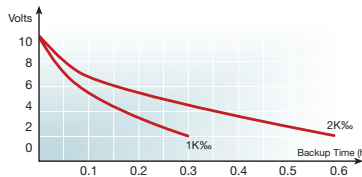
Figure 29. 0.47F - LV Series
