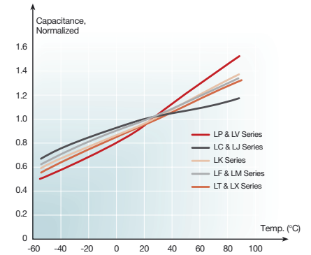
Figure 53. Capacitance Versus Temperature - 1.0F Capacitors
