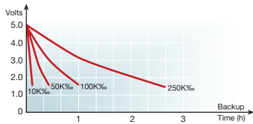
Figure 7. 0.022F – LC, LK, LT, LX Series
