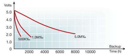
Figure 26. 4.7F - LX & LJ Series
