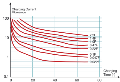
Figure 45. LG Series - 5 Volt Charge
