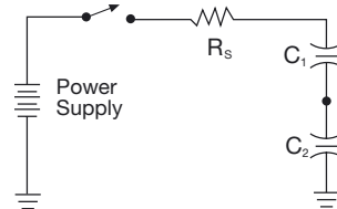
Figure 61. Series Resistor to Limit Charge Current.
