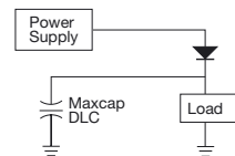
Figure 55. Basic Backup Circuit
