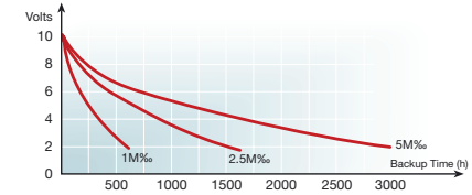
Figure 36. 1.0F - LV Series
