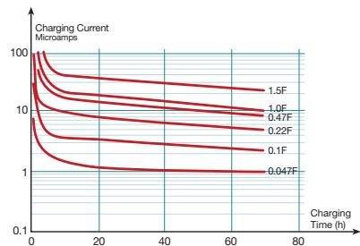
Figure 46. LF Series - 5 Volt Charge
