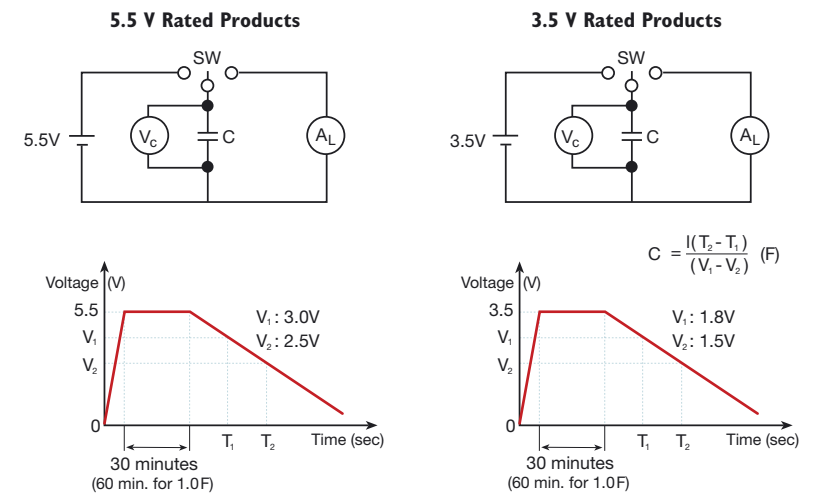
Figure 2. — Discharge Method – LM Series (Surface Mount)
