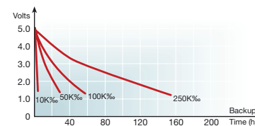
Figure 21. 2.2F – LC, LX, LJ Series
