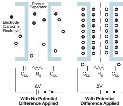
Figure 67. Maxcap DLC Unit Cell Operation
