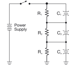
Figure 62. Voltage Divider Using Shunt Resistors for Charge Balancing.
