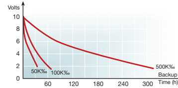
Figure 35. 1.0F - LV Series
