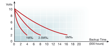
Figure 40. 5.0F - LV Series
