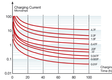
Figure 50. LX Series - 5 Volt Charge
