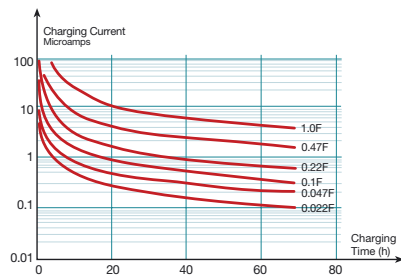
Figure 48. LT Series - 5 Volt Charge
