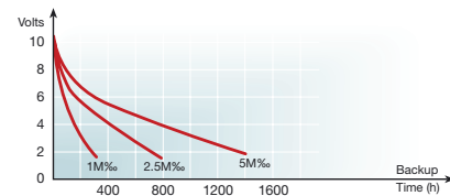
Figure 32. 0.47F - LV Series
