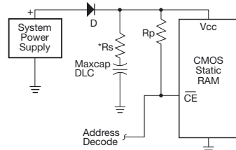
Figure 57. Memory Backup Circuit
