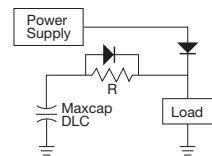
Figure 56. Alternate Backup Circuit
