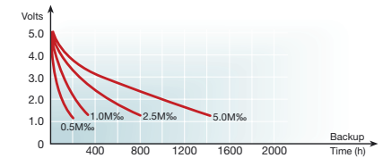
Figure 16. 0.47F – LC, LK, LT, LX, LJ, LM Series
