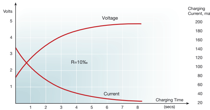
Figure 41. Charging Curves for Maxcap DLC LP055104A
