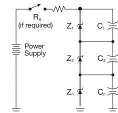
Figure 63. Voltage Divider Using Shunt Zener Diodes for Overvoltage Protection.
